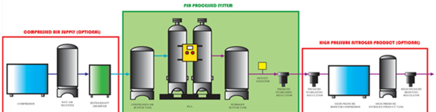
PRESSURE SWING ADSORBERS (P.S.A.)
