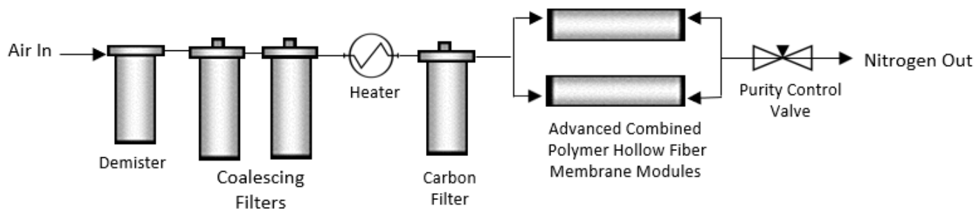
TYPICAL NITROGEN MEMBRANE SYSTEM
