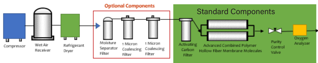
NITROGEN ON THE WALL (NOW) PANELS
