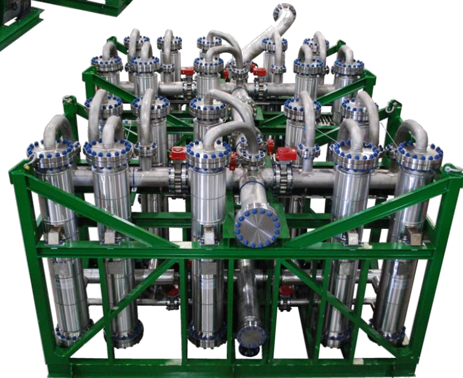
Gas Pre-Treatment Skid with Auxiliary Membrane Skid
